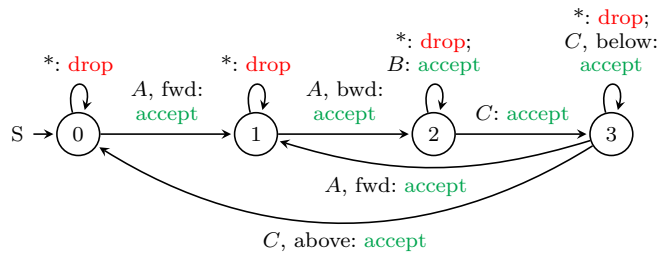
Fig. 5: Finite State Machine for an interaction with an one-off policy A , a periodic policy B and a transient policy C . “fwd” and “bwd” specify the direction of the packet. “below” indicates a packet within the limits of a transient policy. “*” stands for all non-matching traffic.
