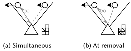
Fig. 2. Types of handovers. The triangle (resp. circles) represents a ground station and its sight cone (resp. satellites). The arrows show the satellites' displacement direction. The available antennas on the ground station are shown by a grid of 4 slots, the 5 th , grey one being dedicated to handovers. The solid (resp. dashed) grey line illustrates an active (resp. candidate) connection. The IGP metrics are shown in grey.
