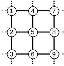
Fig. 1. Illustration of the Walker patterns for a simple constellation of 9 satellites distributed across 3 vertical orbits. A Walker Delta topology exhibits all the links present in the figure, while the dashed grey links connecting the left- and right-most orbits are absent in Walker Star.
