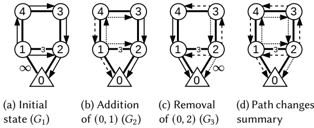
Fig. 4. A simple topology illustrating transient loops triggered by topological modifications. Link metrics are unitary unless specified otherwise. Solid arrows represent paths from each node to Node 0. Dashed (resp. dotted) arrows represent added (resp. removed) paths w.r.t. the previous step.
