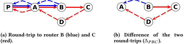
Figure 1: Example of traceroute results with different return paths. P is the probe initiating the traceroute. A , B , and C are routers reported by traceroute. D is a router on the return path, unseen in the traceroute. Solid lines represent the forward paths, dashed the return paths.
