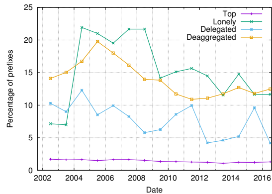
Figure 3: Proportion of selectively announced prefixes by category over time
