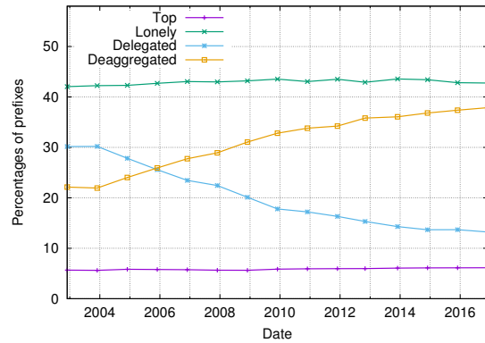
Figure 2: Prefix classification over time
