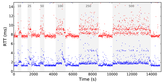
Figure 3: Delays measured from a v2 probe systematically increase when concurrent one-off traceroutes are launched on this probe.
